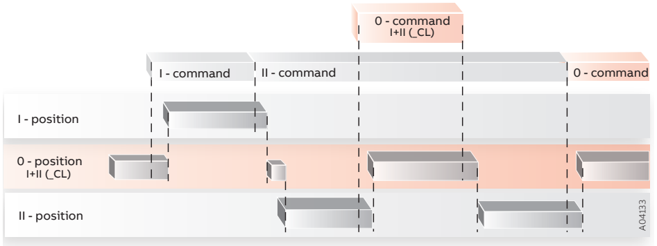
Figure 8.4 Continuous control
