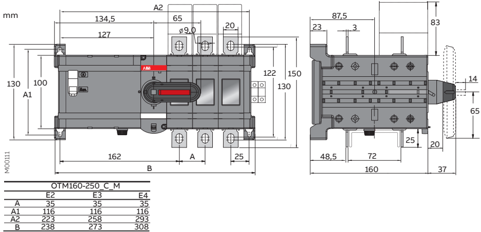
Figure 5.1 OTM160-250E_C_M
