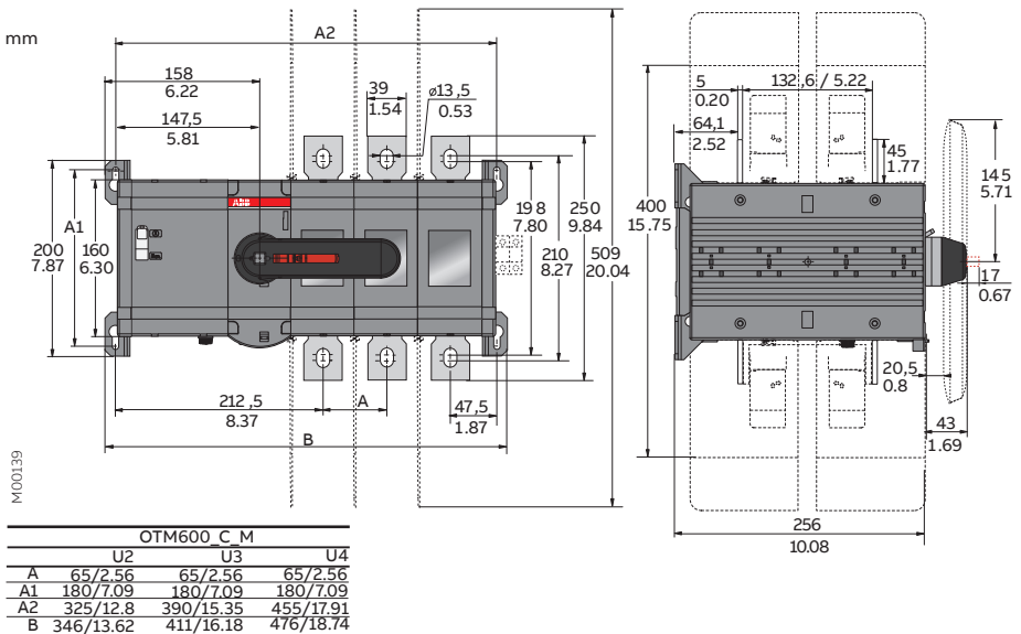
Figure 5.8 OTM600U_C_M
