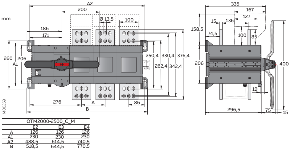
Figure 5.12 OTM2000-2500E_C_M
