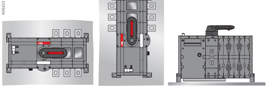
Figure 6.2 Mounting positions
