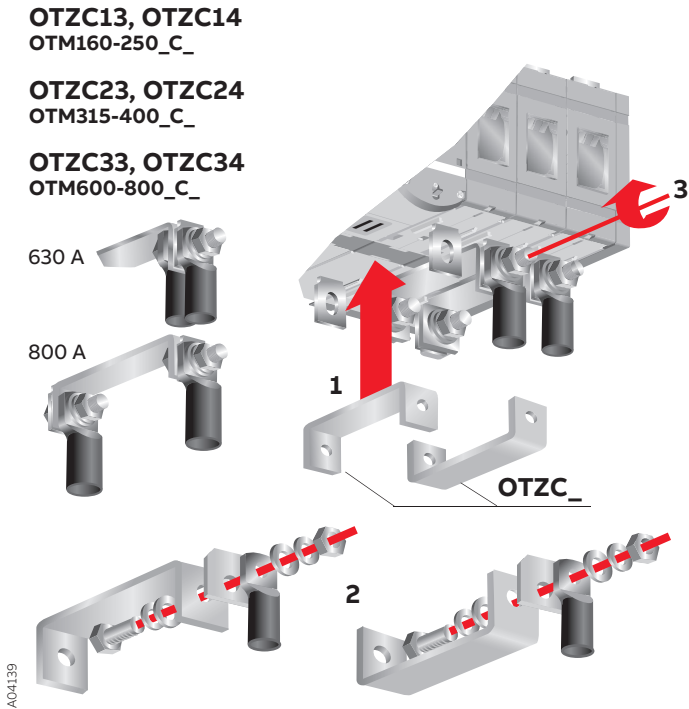
Figure 10.2 Mounting of the bridging bars (type OTZC_) to the motorized change-over switches OTM160-800E_C_
