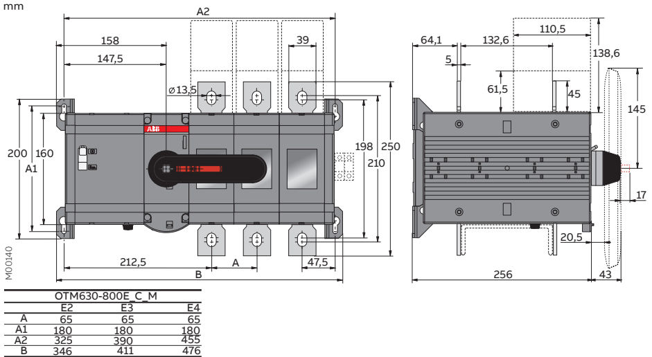
Figure 5.7 OTM630-800E_C_M
