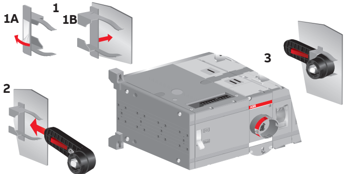
Figure 10.13 Handle and spare fuses can be stored on the motorized change-over switch by mounting the accessory OTVS_
