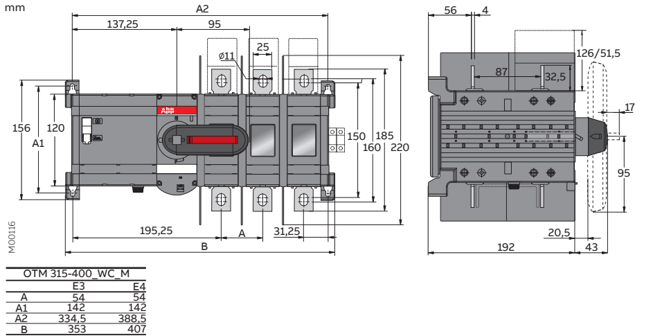
Figure 5.5 OTM315-400E_WC_M
