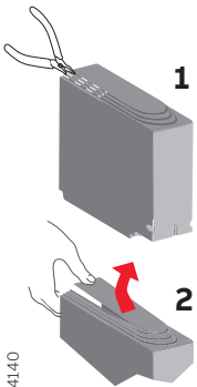
Figure 10.7 Mounting of the terminal shrouds (type OTS_) to the motorized change-over switches OTM160-800E_C_
