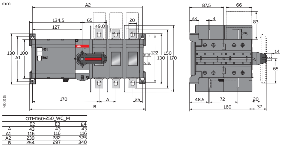
Figure 5.2 OTM160-250E_WC_M
