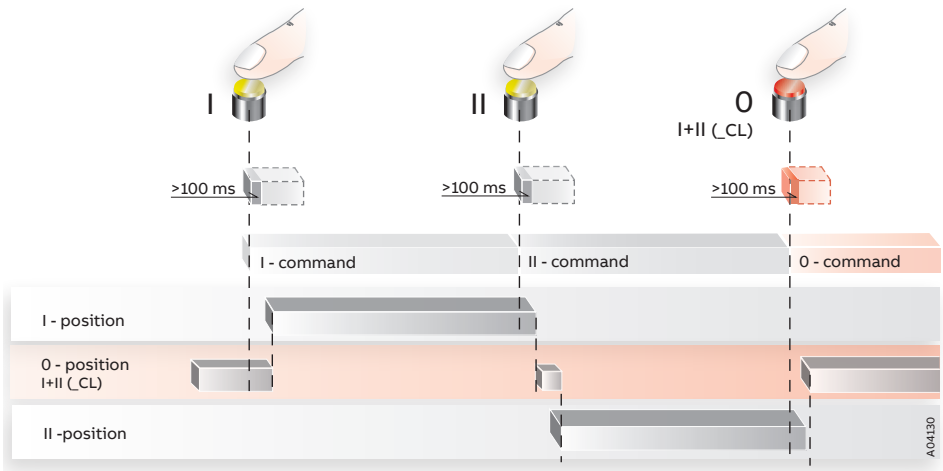
Figure 8.3 Impulse control
