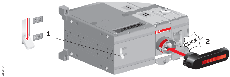
Figure 3.3 Operating the motorized change-over switch manually
