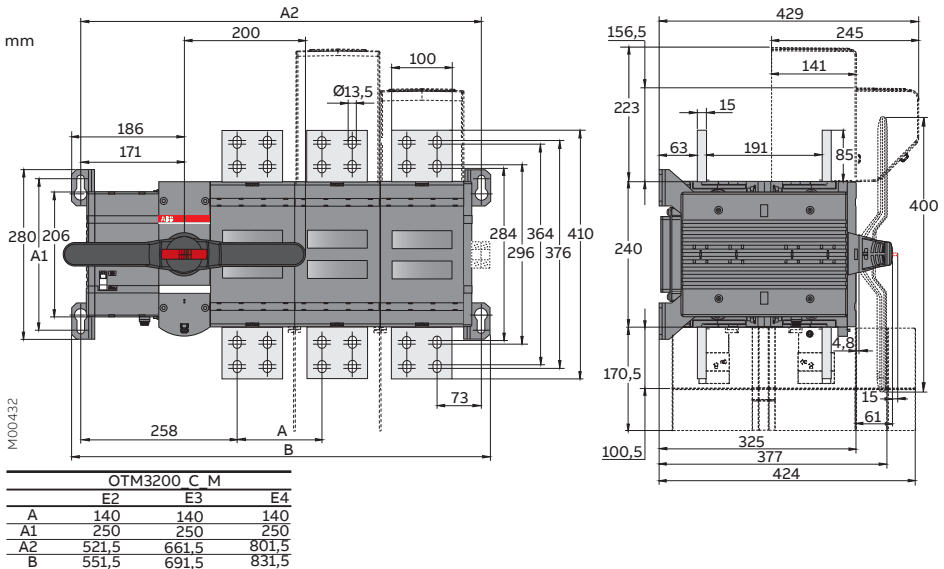
Figure 5.13 OTM3200_C_M
