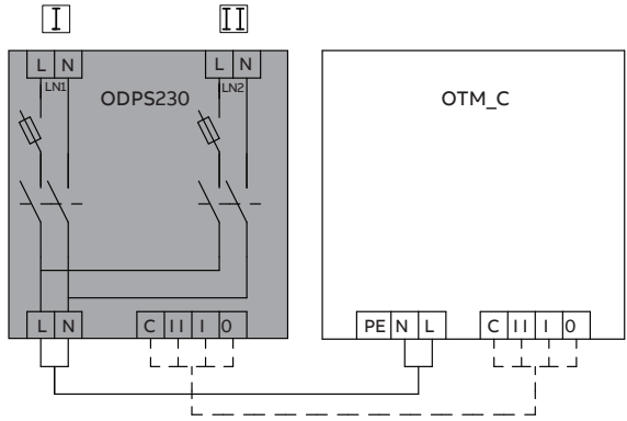
Figure 10.11 The dual power source, type ODPS230. Connection diagram ODPS230.
