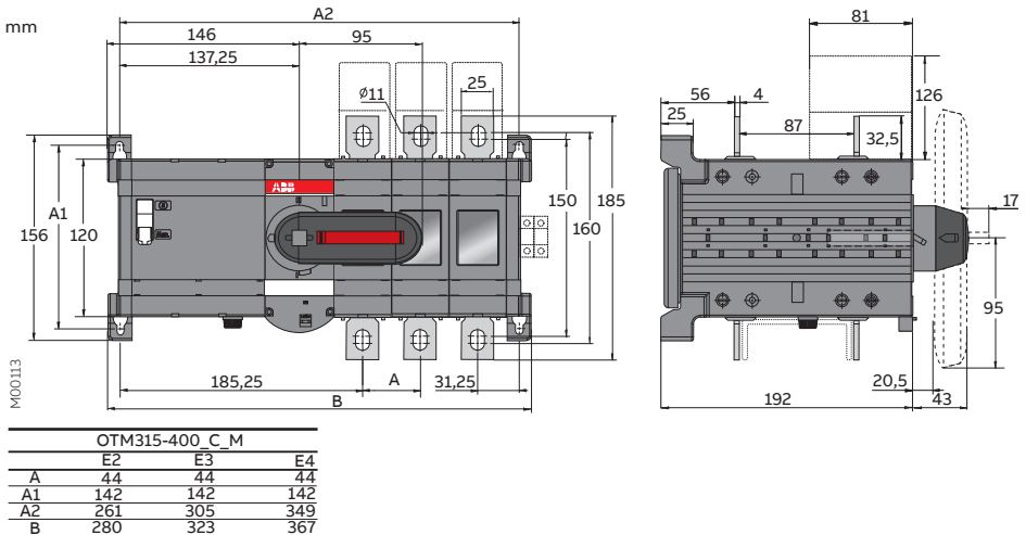
Figure 5.4 OTM315-400E_C_M
