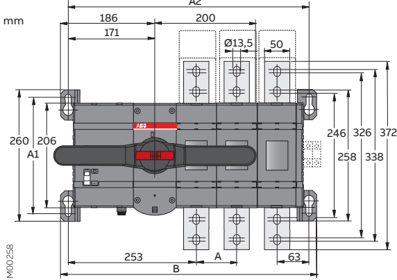
Figure 5.9 OTM1000-1200E_C_M
