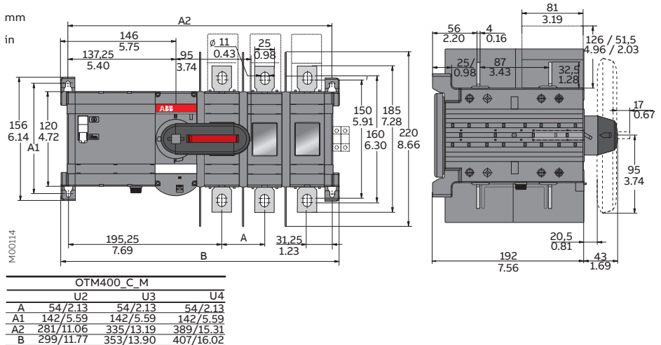
Figure 5.6 OTM400U_C_M
